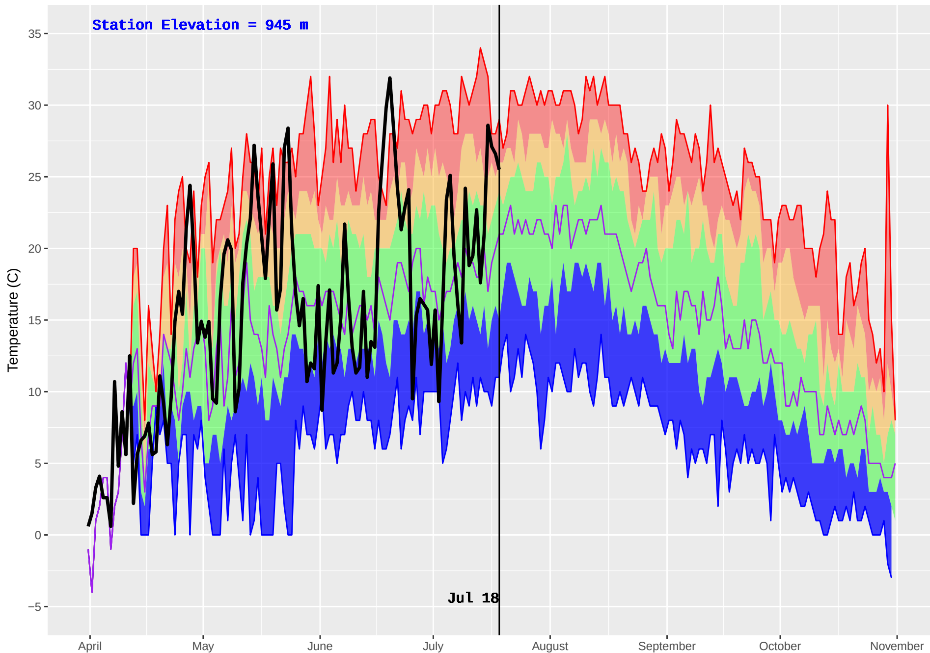
BOWRON HAGGEN (193) : Historical (1986–2016) and Current (2018) Daily Temperature
