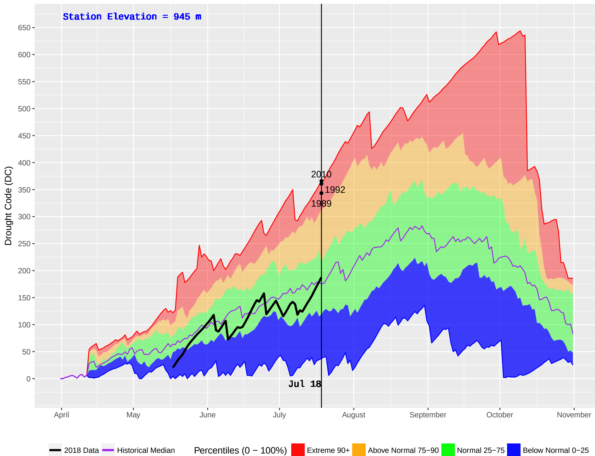
BOWRON HAGGEN (193) : Historical (1986–2016) and Current (2018) Daily Drought Code (DC)
