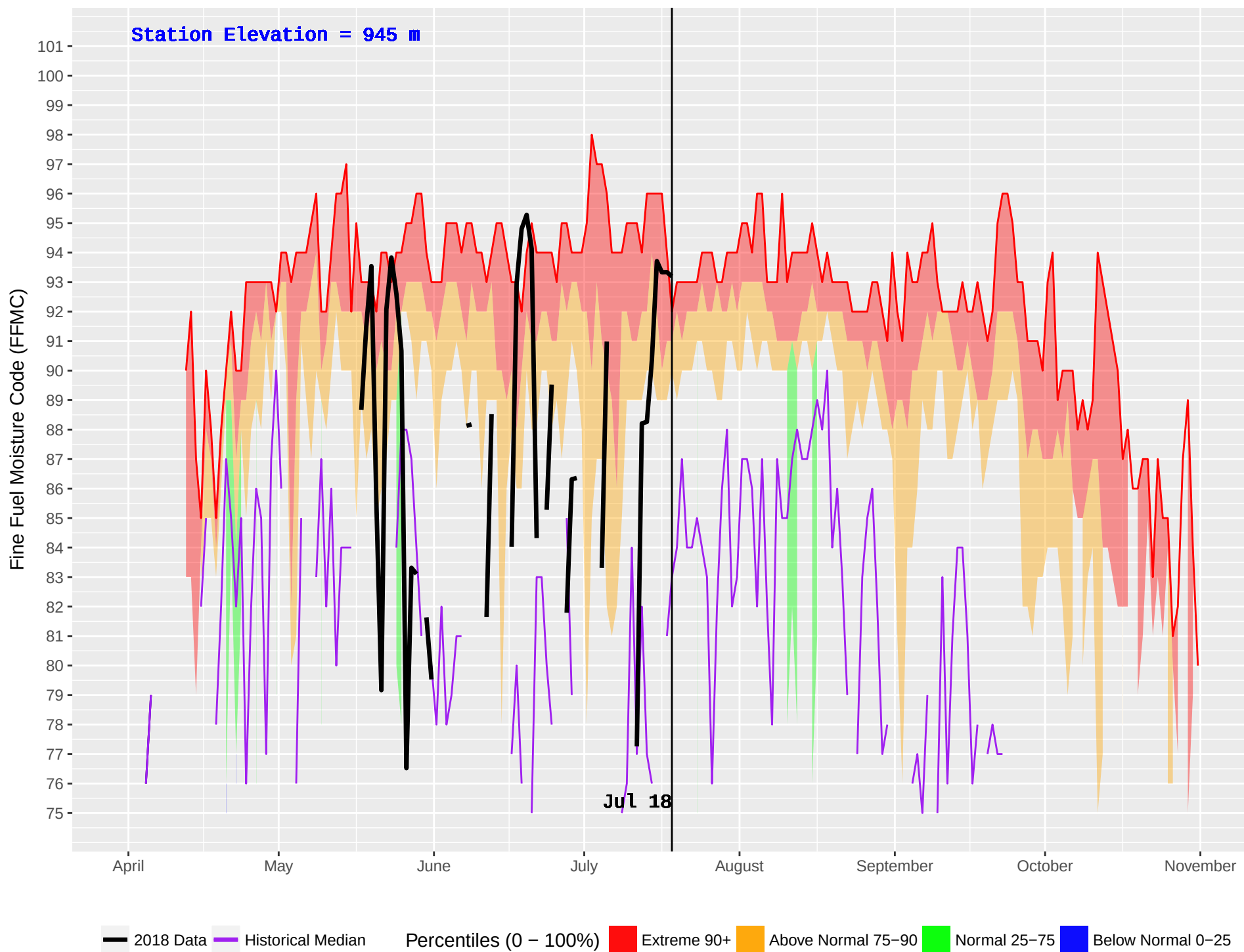
BOWRON HAGGEN (193) : Historical (1986–2016) and Current (2018) Daily Fine Fuel Moisture Code (FFMC)
