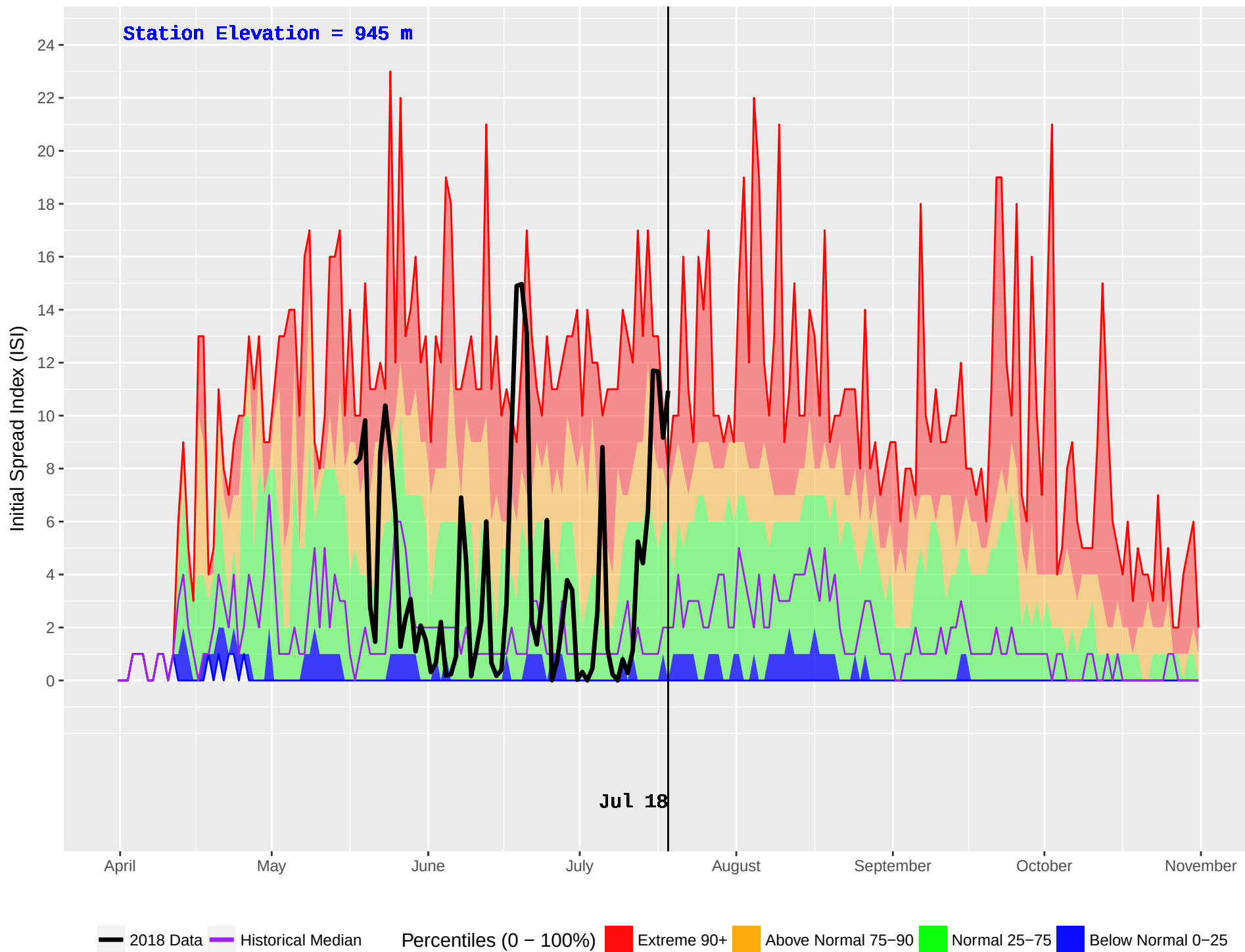
BOWRON HAGGEN (193) : Historical (1986–2016) and Current (2018) Daily Initial Spread Index (ISI)
