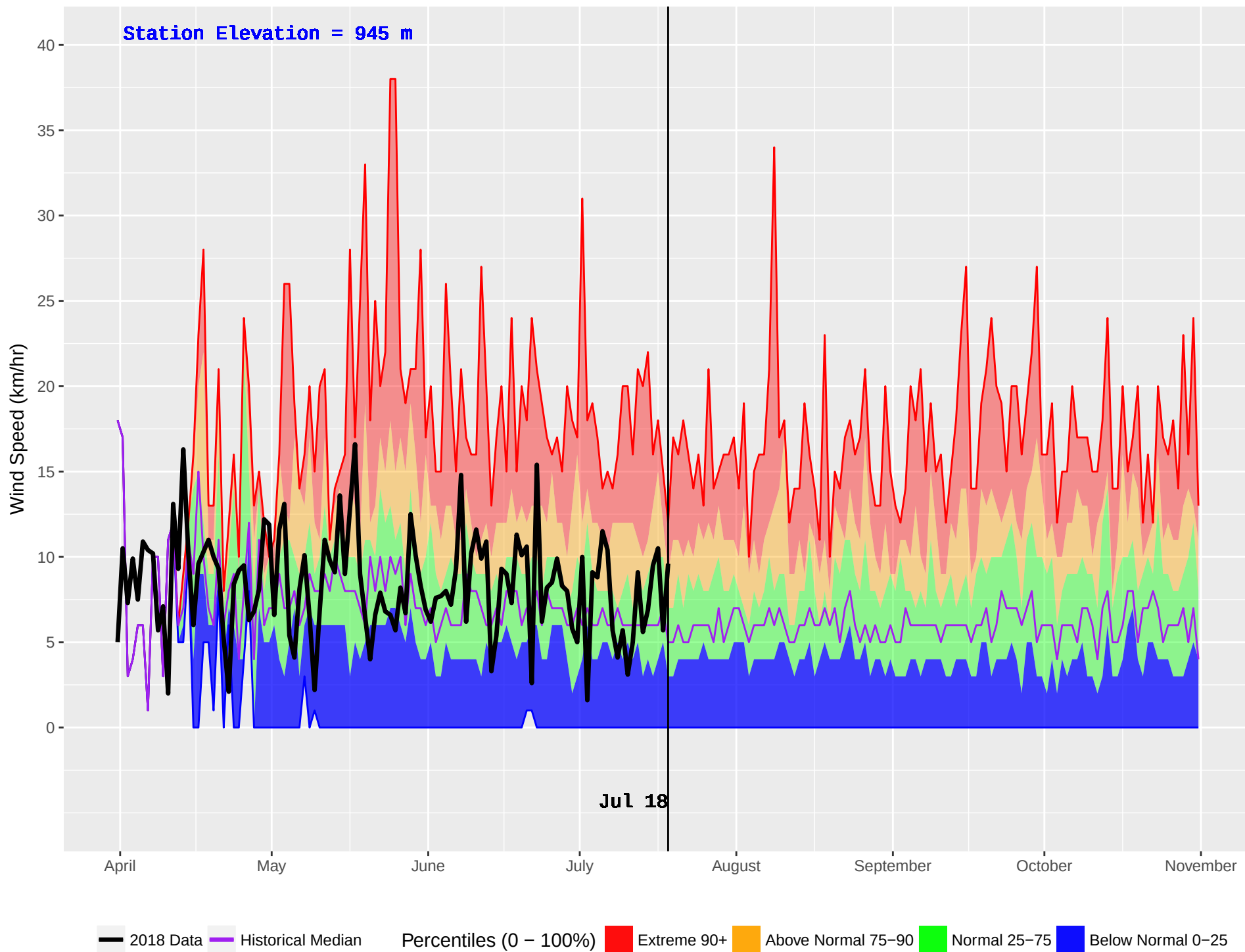
BOWRON HAGGEN (193) : Historical (1986–2016) and Current (2018) Daily Wind Speed
